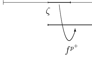
Fig.1 - Singly returning, singly periodic \zeta
