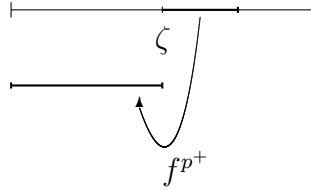
Fig.2 - Singly returning, eventually aperiodic \zeta
