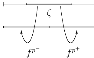
Fig.3 - Doubly returning, doubly periodic \zeta (no switches)
