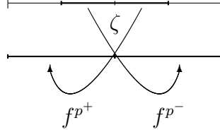
Fig.5 - Doubly returning \zeta with two switches
