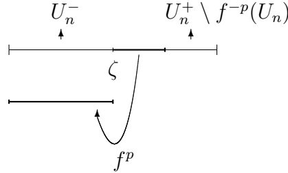
Fig.6 - Q_p = U_n^- \cup (U_n^+ \setminus f^{-p}(U_n))
