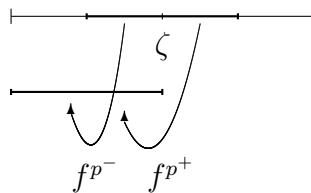
Fig.4 - Doubly returning \zeta with one switch
