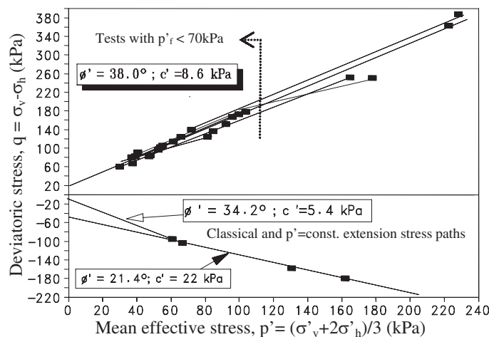
Figure 29. Failure envelopes from triaxial tests in compression and extension on undisturbed samples.
