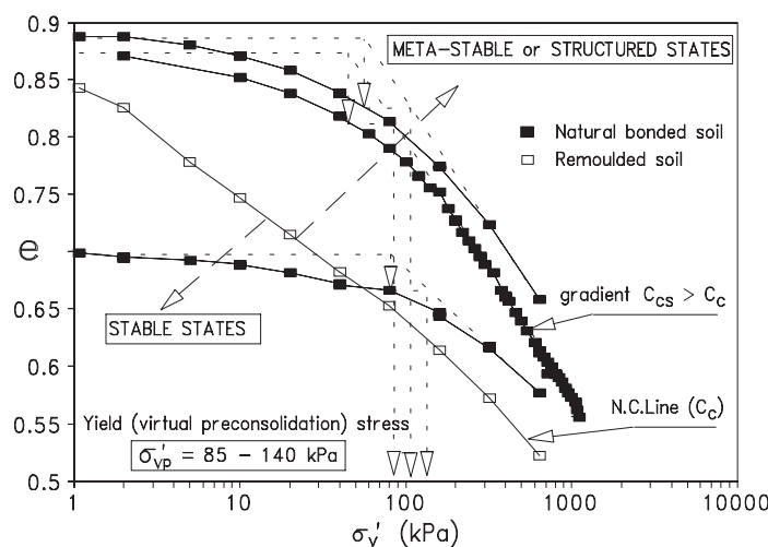
Figure 22. Oedometer curves – state definition.
