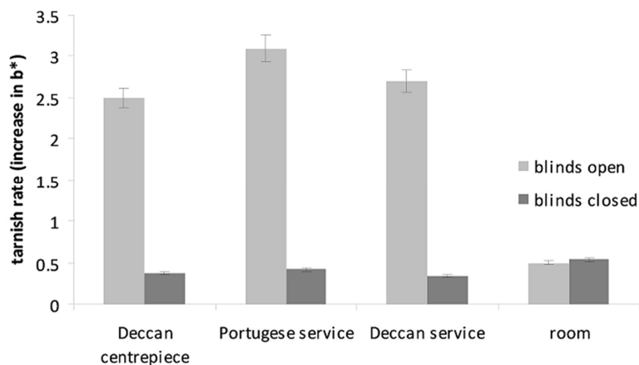
FIG. 5 – Silver tarnish.
