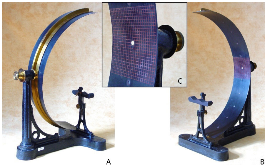
FIG. 16 - Landolt perimeter (Physics collection of the Museum of Science, Inv. 000375): A – The outer side, divided into degrees; B – The blackened inner side of the arc; C – The grid spaced in half degrees.
