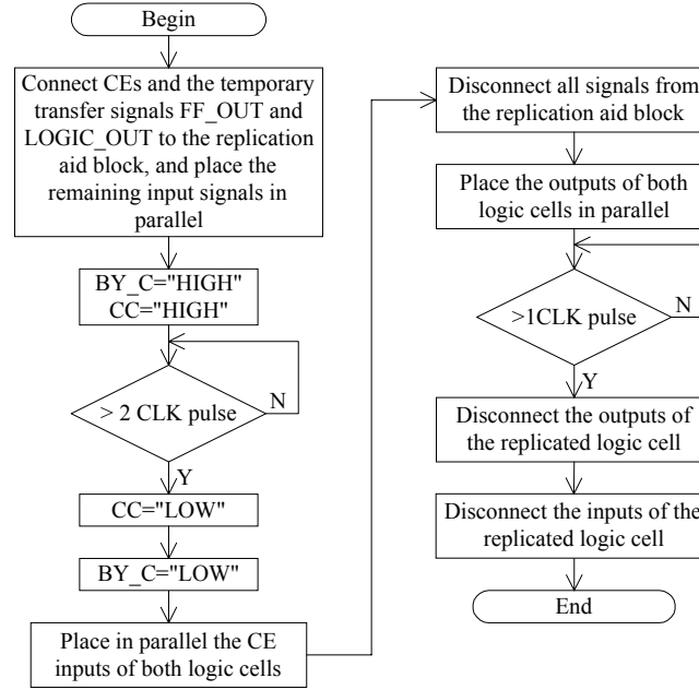
Fig. 3. Replication process flow.
