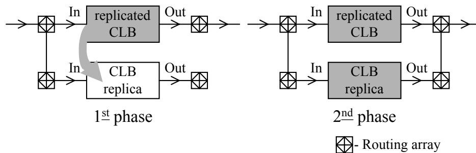
Fig. 1. Two-phase CLB replication process.
