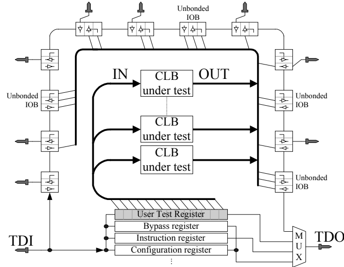
Fig. 4. Test of CLBs through the BS infrastructure.
