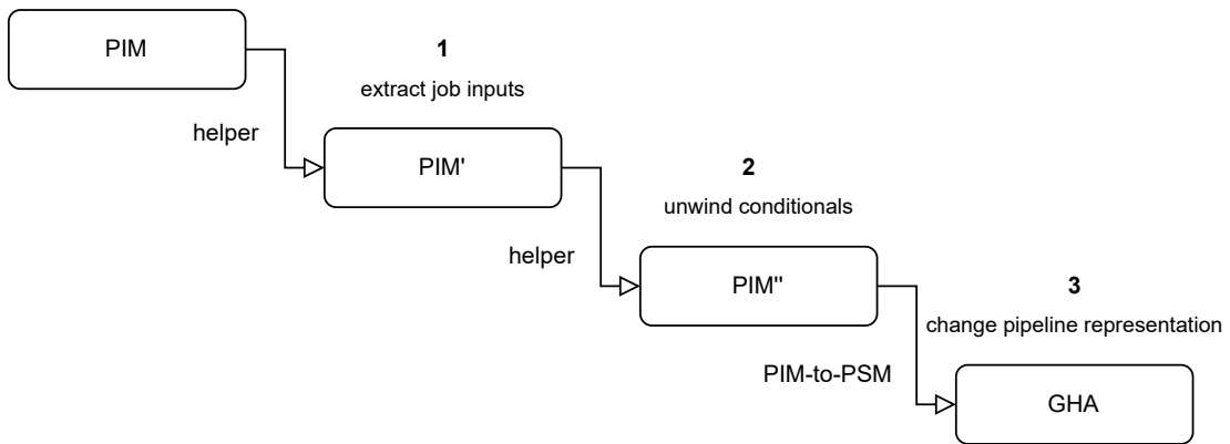
Figure 6.1: PIM-to-GHA transformations.
