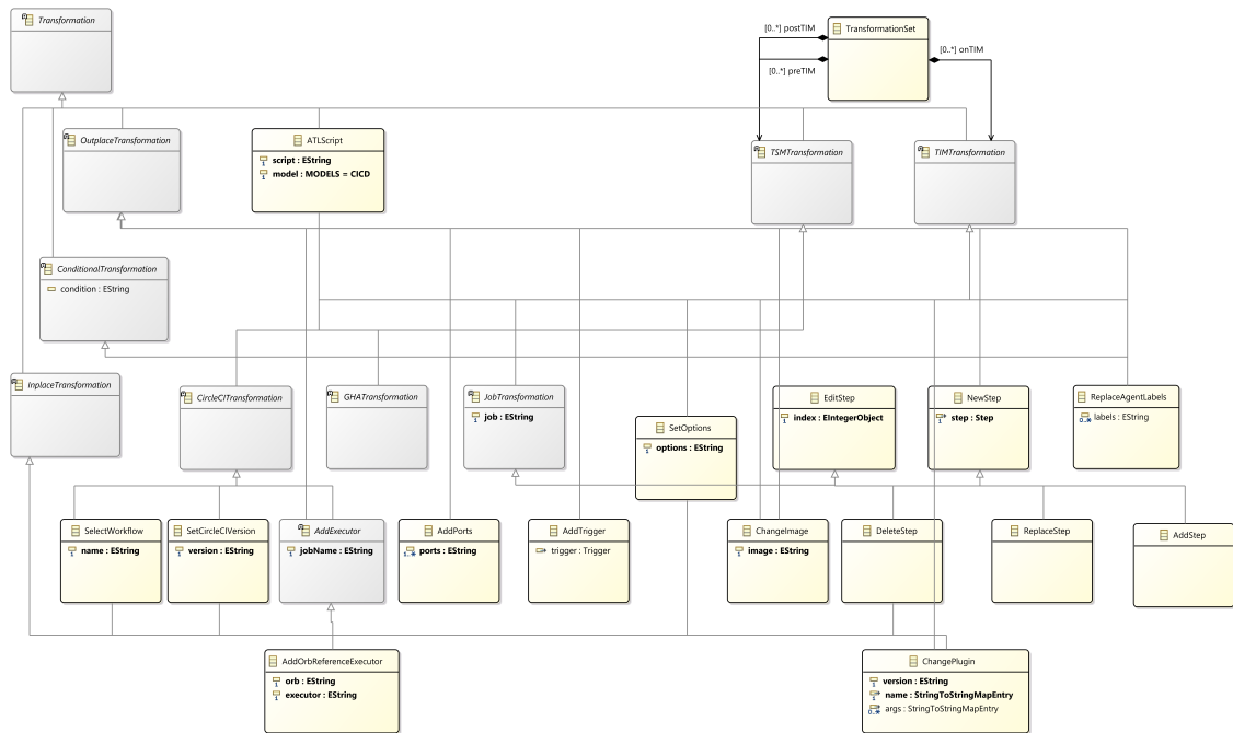
Figure 7.2: TDSL meta-model.
