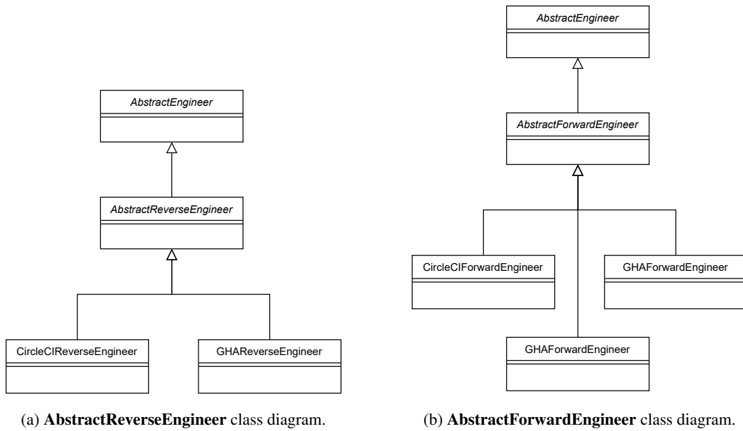
Figure 8.1: AbstractEngineer class diagrams.
