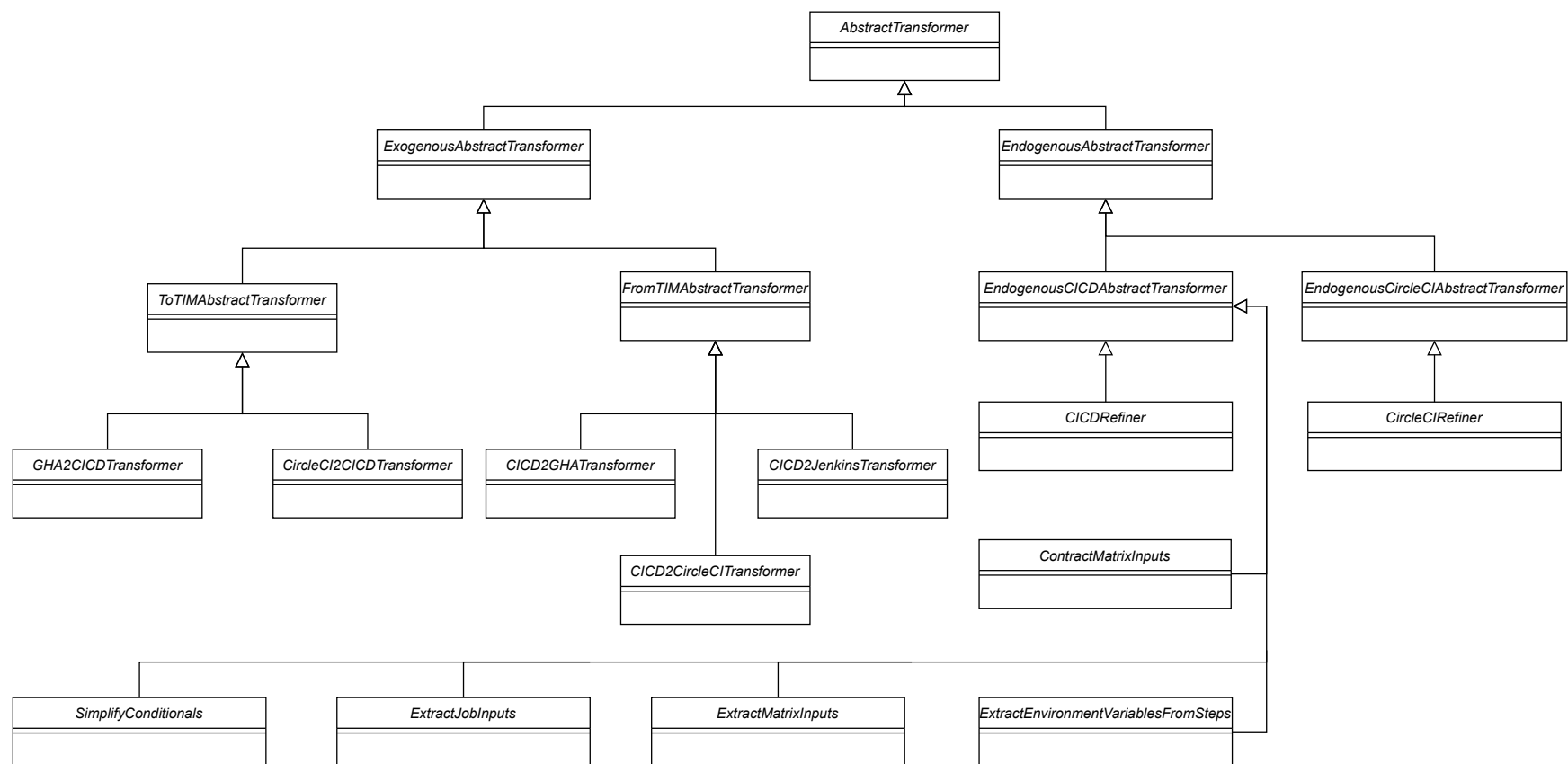
Figure 8.2: AbstractTransformer class diagram.
