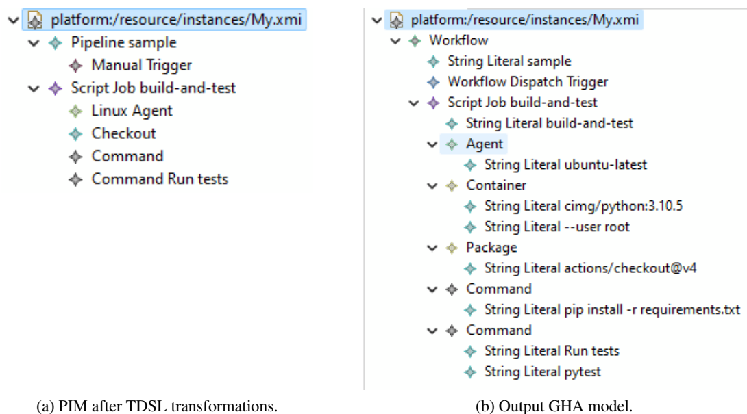
Figure 4.4: PIM and GHA model representations of output pipeline.
