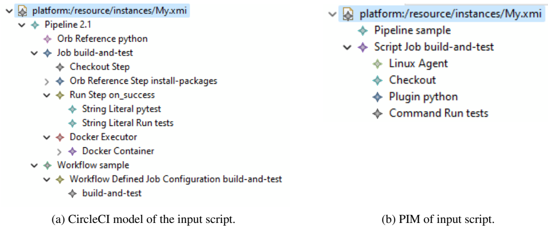
Figure 4.3: CircleCI model and PIM representations of input pipeline script.
