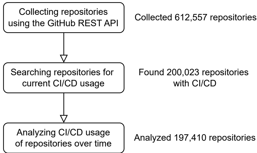
Figure 3.1: Data collection process.
