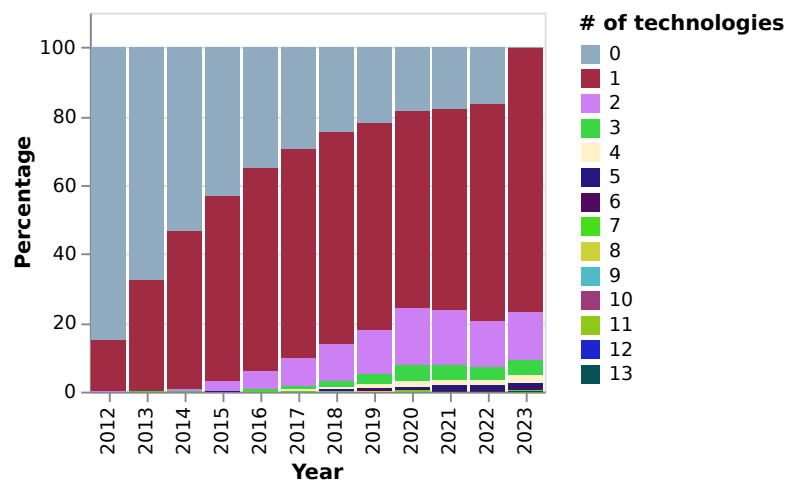
Figure 3.5: Percentage of active repositories using at most a given number of platforms in a given year by year.
