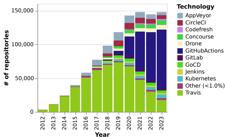
Figure 3.2: Number of active repositories where each platform was detected by year.
