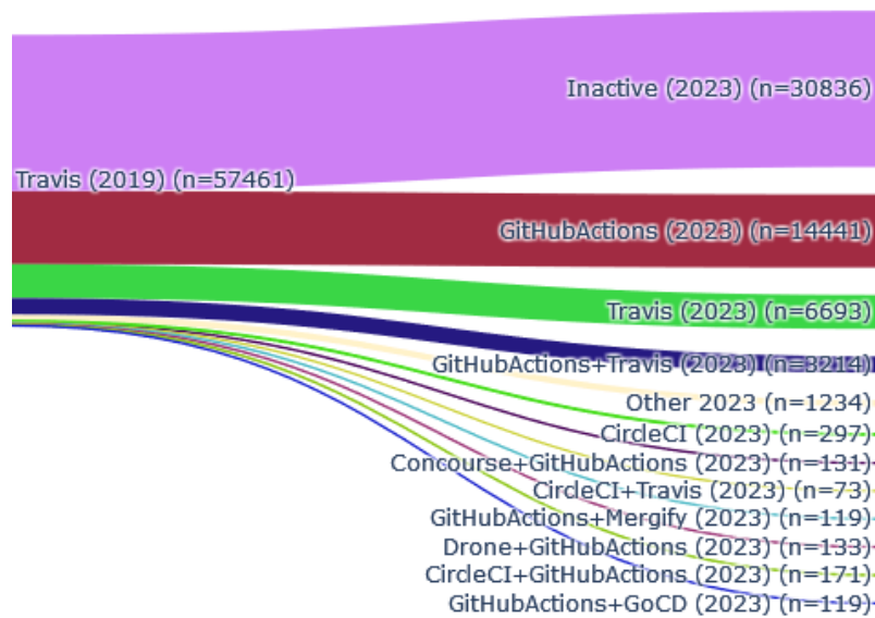
Figure 3.4: CI/CD platform stack transitions from repositories solely using Travis CI in 2019.
