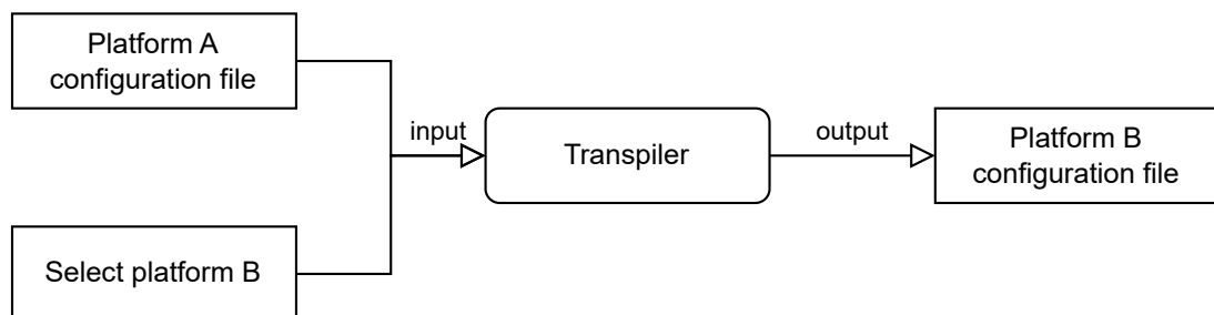
Figure 4.1: Automatic CI/CD migration tool.
