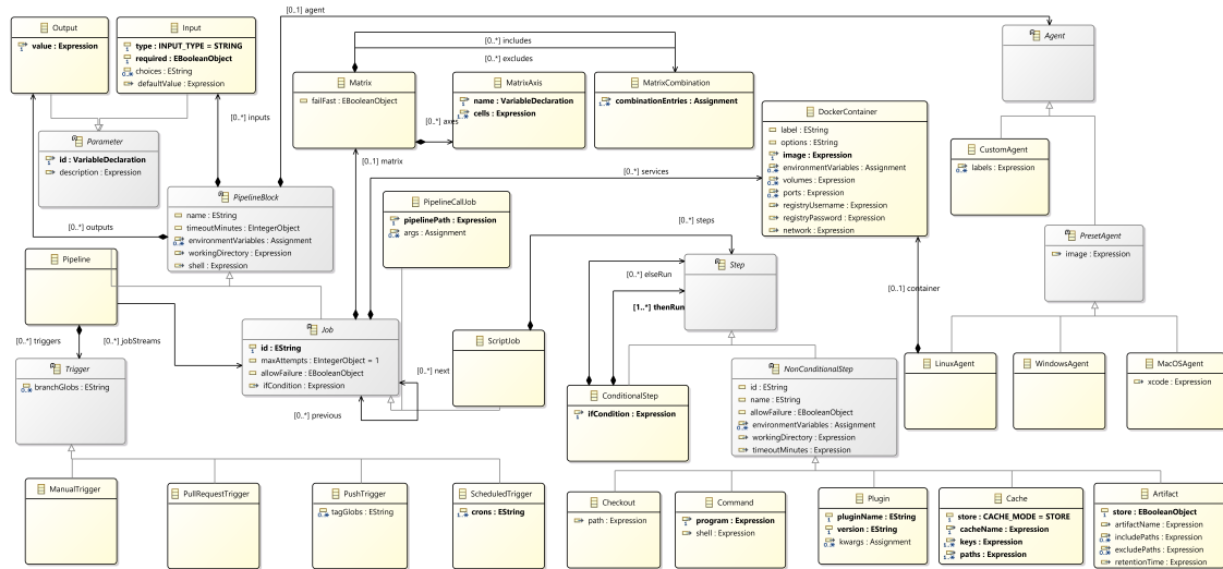
Figure 5.1: Truncated PIMM (missing Expressions , VariableDeclaration , and enumerated classes).
