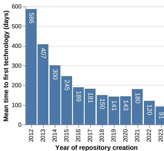
Figure 3.3: Mean time in days to first CI/CD platform detection by repository creation year.
