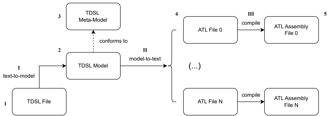
Figure 7.1: TDSL reengineering process.
