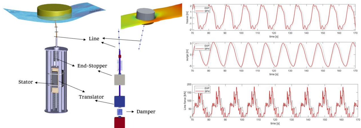
Figure 2: Schematics depicting the parts of the WEC (Waters (2007) Copyright 2007 AIP Publishing LLC.) and their counterparts in the SPH model (left). Comparison of the numerical and experimental heave, surge, and line force(right) (Tagliafierro 2021a).
