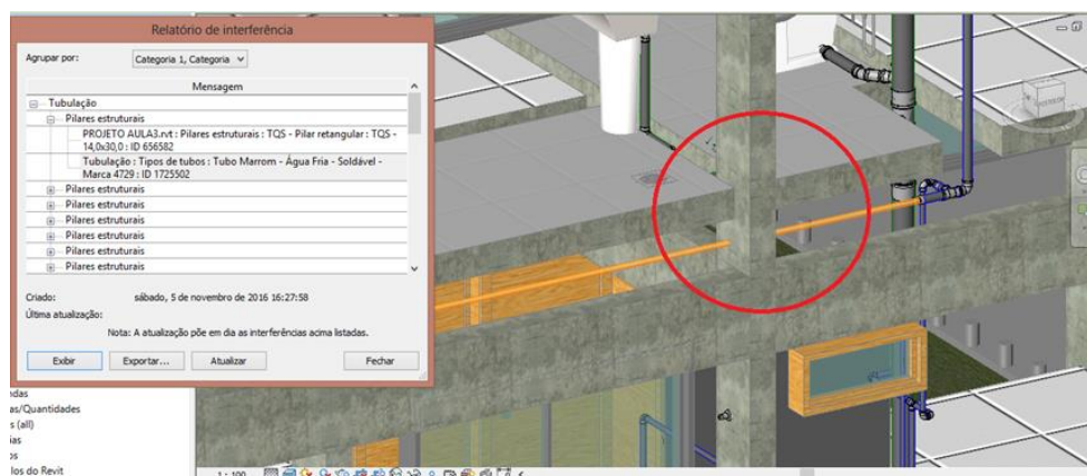
Figure 1: Clash detection
