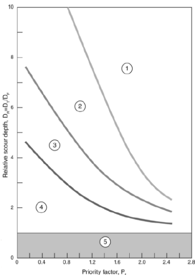
Figure 30: Scour risk rating (Highways Agency, 2012).
