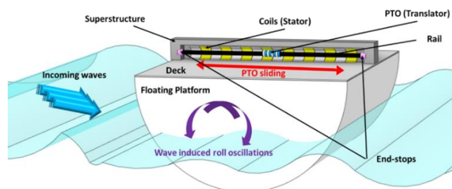
Figure 23: Schematic of the E-Motions and its operation mode.
