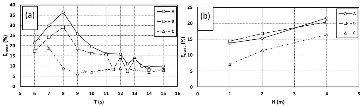
Figure 18: Hydraulic efficiency of the OTD component by (a) wave period with a fixed wave height (1 m) and (b) by wave height with a fixed wave period (resonant period of each tested geometry).
