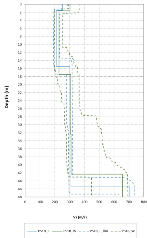
Figure 3: Seismic Profile from joint inversion of MASW + HSR. From Lopes et al. (2018)
