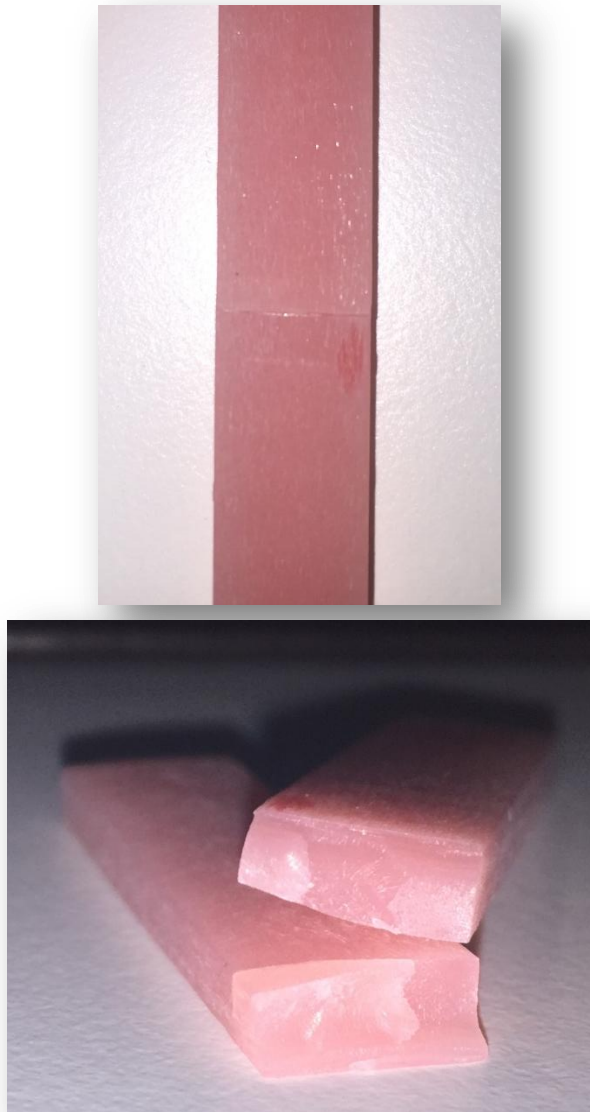
Figure 6. Brittle fracture
