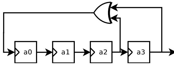
Figure 4.3: MLS generator block diagram.
