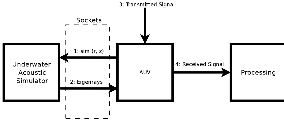
Figure 6.1: Simulation process.
