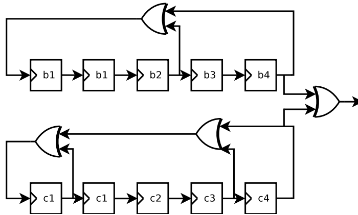
Figure 4.4: Gold sequence generator block diagram.
