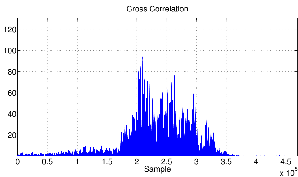
Figure 8.3: Cross correlation with a signal transmitted in Matosinhos on the 11/Jul/2014.
