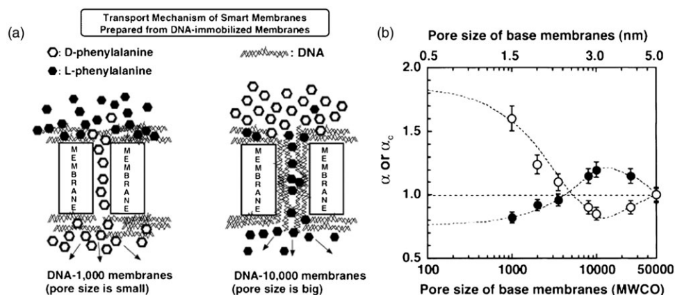
Fig. 5 The mechanism (a) and the separation factor (b) in the permeate ( \circ ; \alpha_c ) and concentrate ( \bullet ; \alpha_c ) solutions regulated by the MWCO of the base membranes in optical resolution of D/L-Phe by immobilized DNA membranes at pH 7.0 and 25°C. \alpha_c is defined as the concentration ratio of D-Phe to L-Phe in the feed solution after starting the experiment. (Reproduced with permission from ref. 114 and 115. © 2003 and 2005 Elsevier.)
