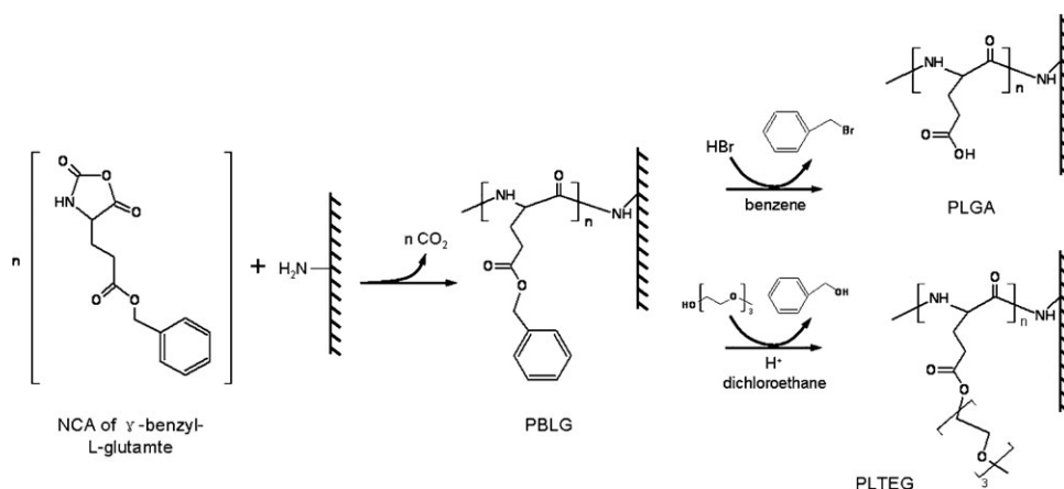
Fig. 11 Steps for preparation of PLGA and PLTEG membranes by debenzylation or ester exchange reaction from poly( \gamma -benzyl-L-glutamate). (Reproduced with permission from ref. 104. © 2002 Elsevier.)
