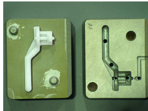
Fig. 2. Resin mould for thermoplastic injection with an injected part in polyacetal.
