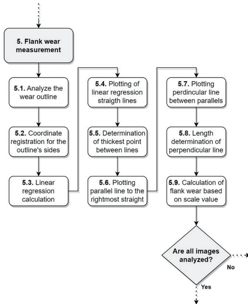
Figure 14: Flowchart showing the intermediary steps of main step 5 devoted to the flank wear measurement
