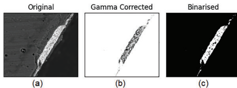
Figure 7: Steps to achieve the initial binarization of an SEM image: (a) original image, (b) image with applied gamma correction, and (c) binarized image
