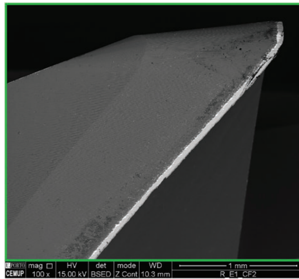
Figure 5: Analysis region (delineated in green) of an SEM image of an end-mill's flank
