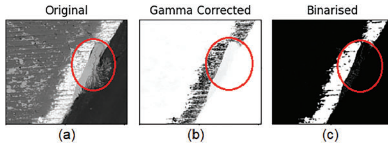
Figure 8: Binarization of an SEM image with adhered material, which is shown inside the red circle: (a) original SEM image, (b) gamma corrected image, and (c) binarized image, exhibiting a dark spot on the adhesion area
