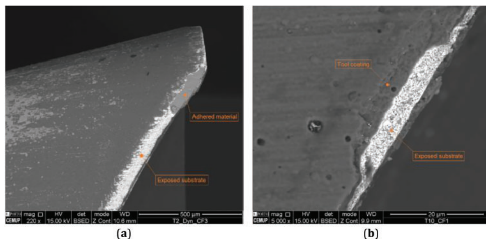
Figure 2: SEM images obtained for tool wear analysis: (a) TiAlN/TiN coated end-mill used in the machining of titanium alloys, and (b) TiAlN coated end-mill used in the machining of stainless steel alloy
