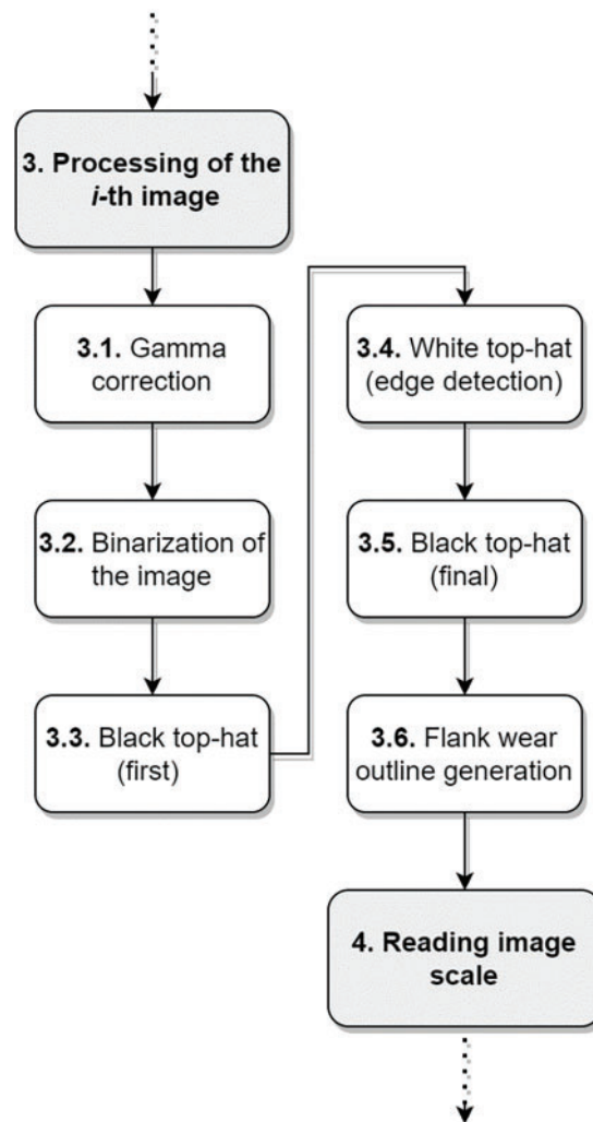
Figure 6: Flowchart showing the intermediary steps of the main step 3 for processing an input image
