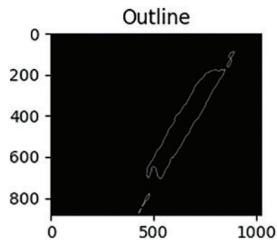
Figure 11: Outline of the identified flank wear generated by the developed algorithm (the x and y axes' numbering represents the input image's pixels)
