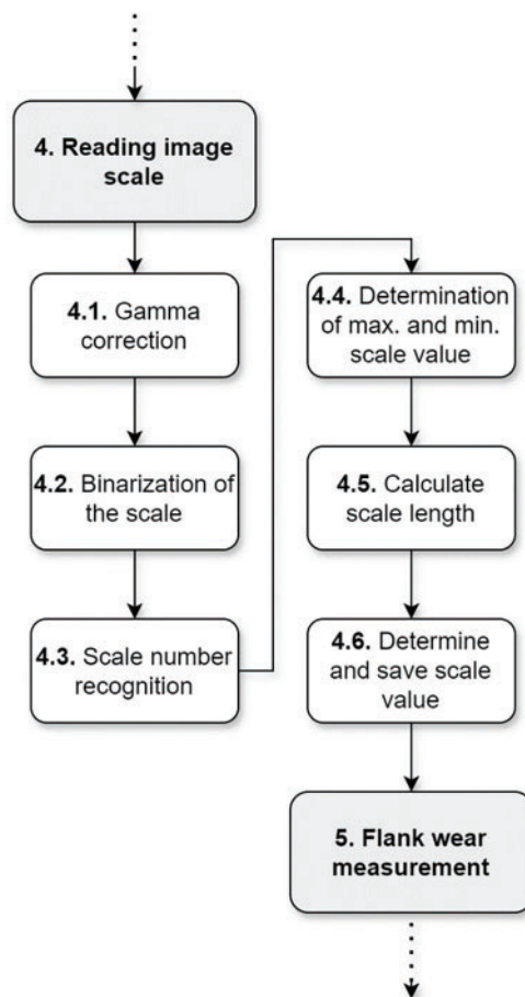
Figure 12: Flowchart showing the intermediary steps of the main step 4 used to obtain the image scale under analysis
