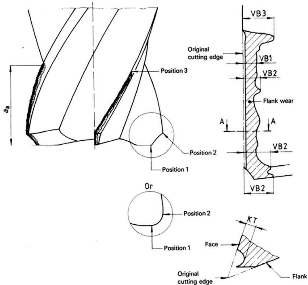
Figure 1: Types of wear on milling cutters (adapted from ISO 8688-2)
