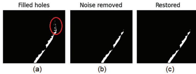
Figure 10: Application of morphological operations to an SEM image of a tool worn: (a) after the application of a black top hat filter, with some wear on the tool's top being visible in the red delineated region, (b) after the application of a white top hat filter to remove the wear pattern on the tool's top, and (c) after the application of a final black top hat filter to clean the wear pattern further
