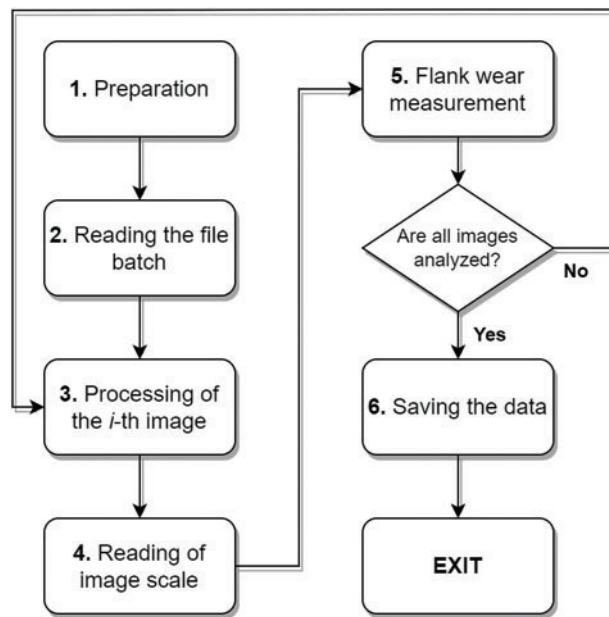
Figure 4: Flowchart of the developed flank wear measurement algorithm
