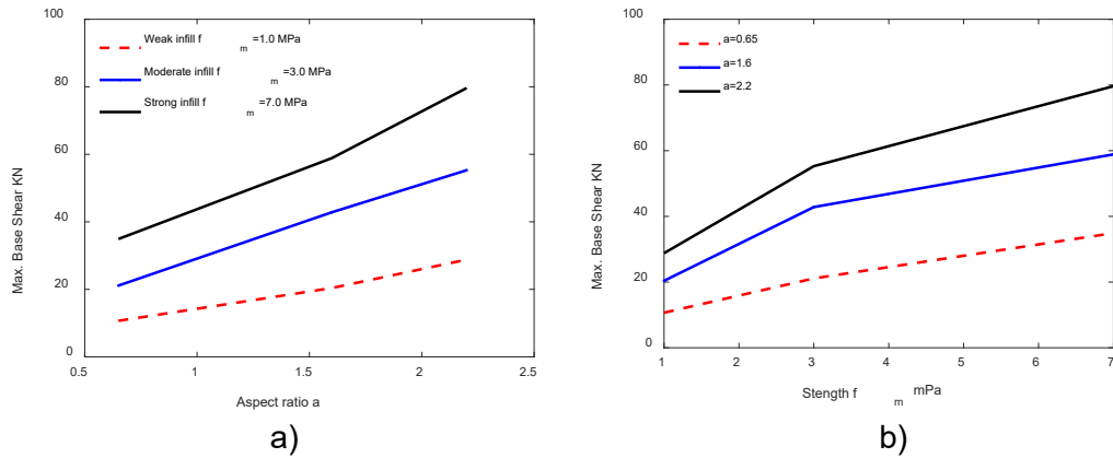
Figure 6 Variation of drift corresponding to maximum strength with a) aspect ratio b) strength of masonry.
