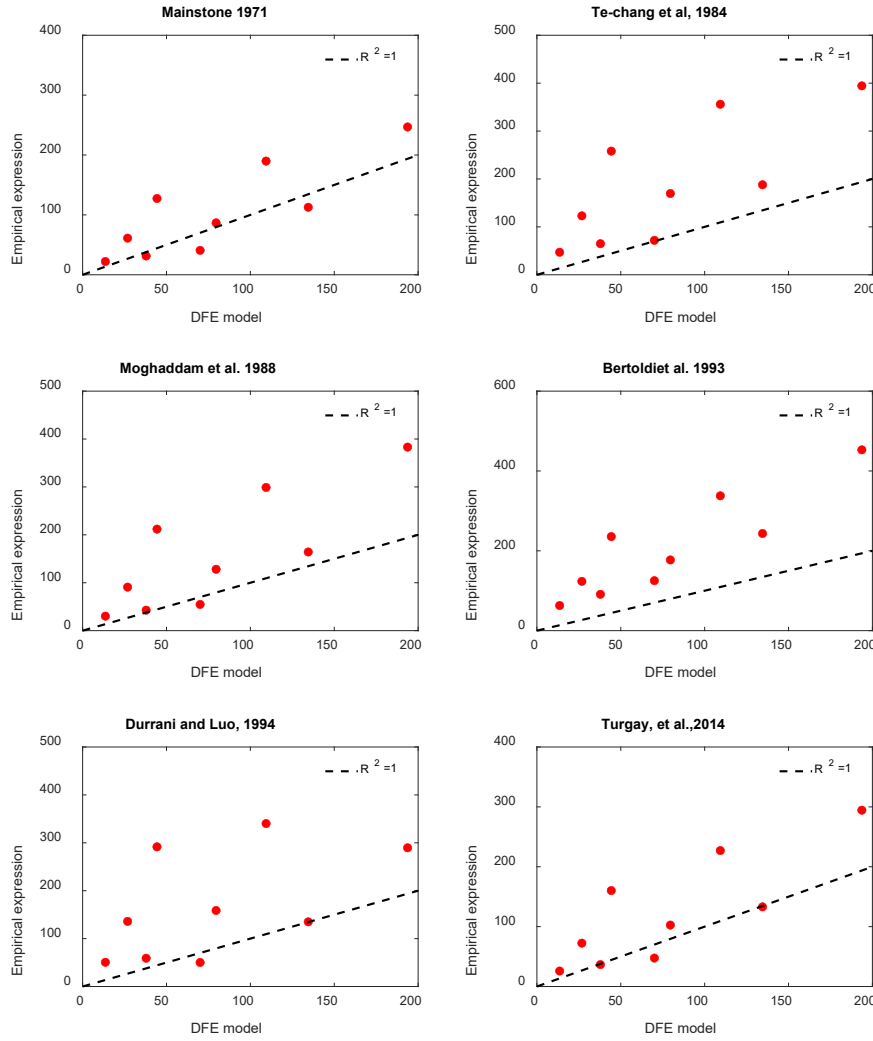
Figure 7 Scatter plots representing estimated infill contribution in terms of strength using different empirical expressions versus the strength obtained from the detailed finite element model.
