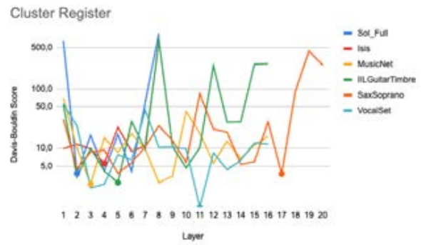
(b) Clustering on Register
