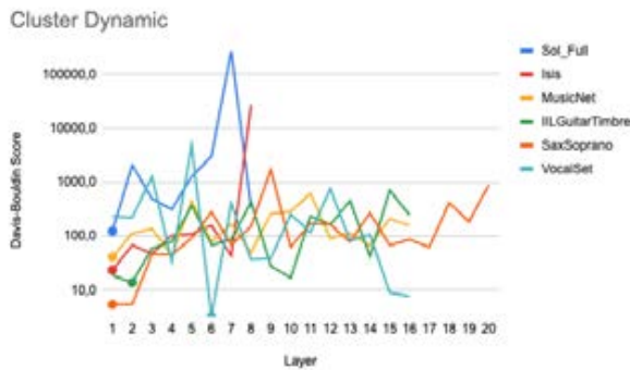
(c) Clustering on Dynamic
