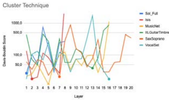
(a) Clustering on Technique
