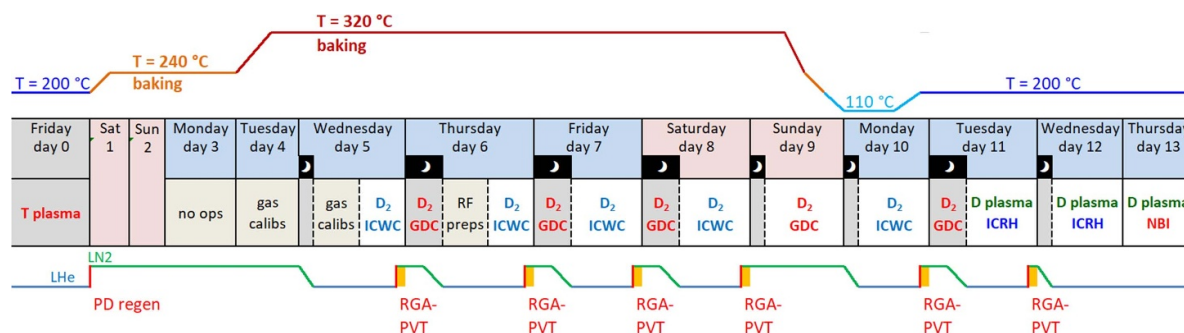
Figure 23. Experimental sequence of tritium removal after the JET-ILW T and DTE2 campaigns in 2021/22, with a combination of different tritium cleaning techniques targeting different PFC areas. The upper line shows the evolution of the vessel wall temperature with baking phase and the lower line indicates the condition of divertor cryo-pumping (PD = pumped divertor; LHe and LN2 = phases with cryo-panels at liquid He and liquid nitrogen temperatures, respectively). The moon shaped icons indicate that glow discharge cleaning (GDC) cycles and subsequent cooling down of cryo-panels to LHe were executed overnight. Reproduced from [112]. © 2023 The Author(s). Published by IOP Publishing Ltd on behalf of the IAEA. All rights reserved. CC BY 4.0 .
