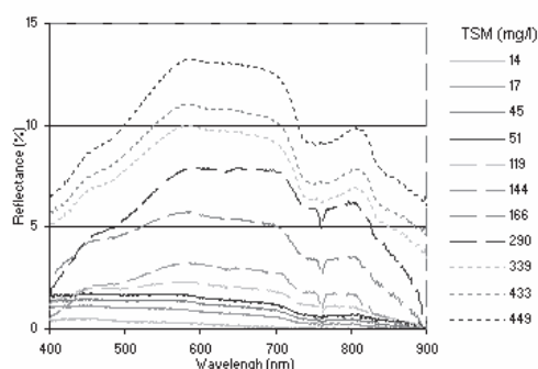
Figure 9: Relationship between TSM and seawater reflectance
