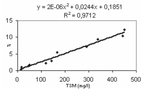
Figure 8: Polynomial model from ASTER VNIR1 data
