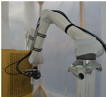
XLIII Molde de Malha Metal, ETH—Institute of Technology in Architecture, Zurique.
