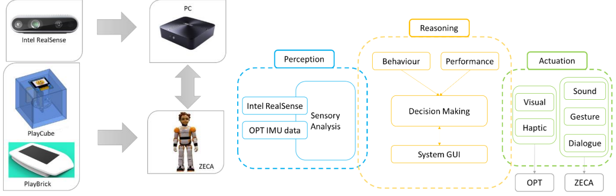
Figure 1: On the left: the proposed system. On the right, the behavioural architecture is depicted – the perception (blue), Reasoning (yellow), and Actuation (green) layers (Vinícius Silva et al. 2019).
