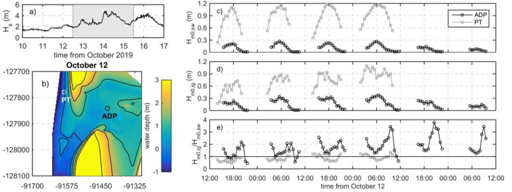
Figure 1. Time-series of significant wave height (a) recorded by Sines wave buoy. Digital elevation model obtained with the topographic survey performed on October 12 (b) and spatial locations of the acoustic Doppler current profiler (ADP) and the pressure transducer (PT). Water depth is referred to mean sea level and the horizontal coordinates are referred in the ETRS89 PT-TM06 system. Time-series of significant short-wave (c) and infragravity wave (d) height and the ratio between significant infragravity and short wave heights (e) at the ADP (circles) and PT (squares) locations.
