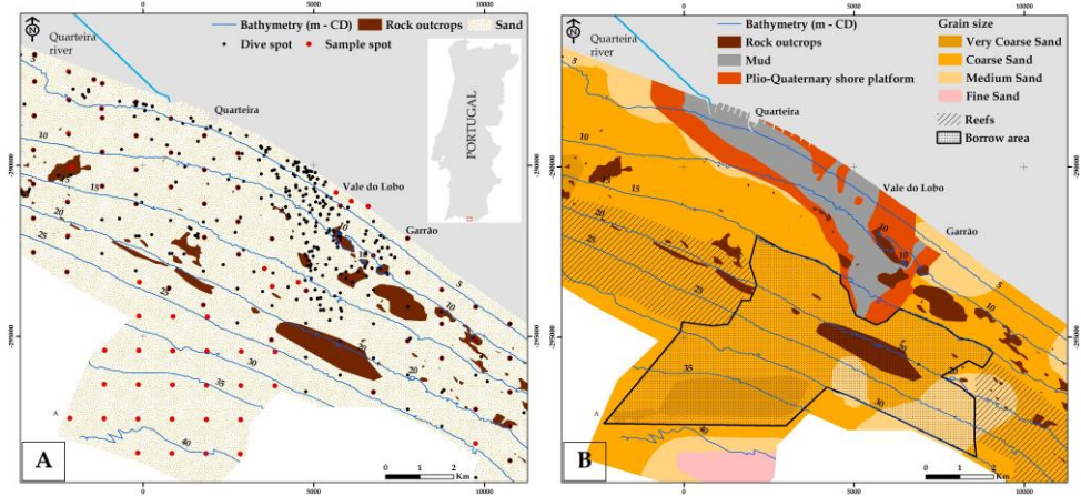
Figure 1 – A) Map of seafloor based on side scan sonar interpretation, location of dive spots and sand sample spots; B) Granulometric sand spatial distribution and borrow area location.
