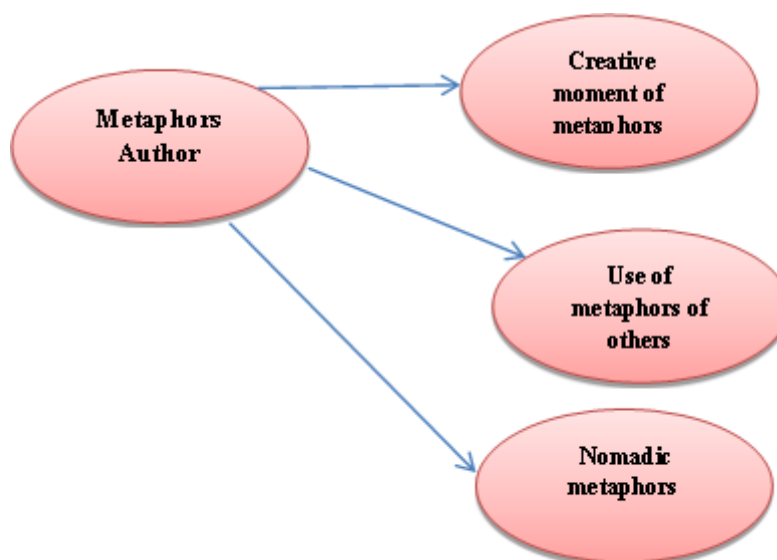
Figure 1. Authoring metaphors
