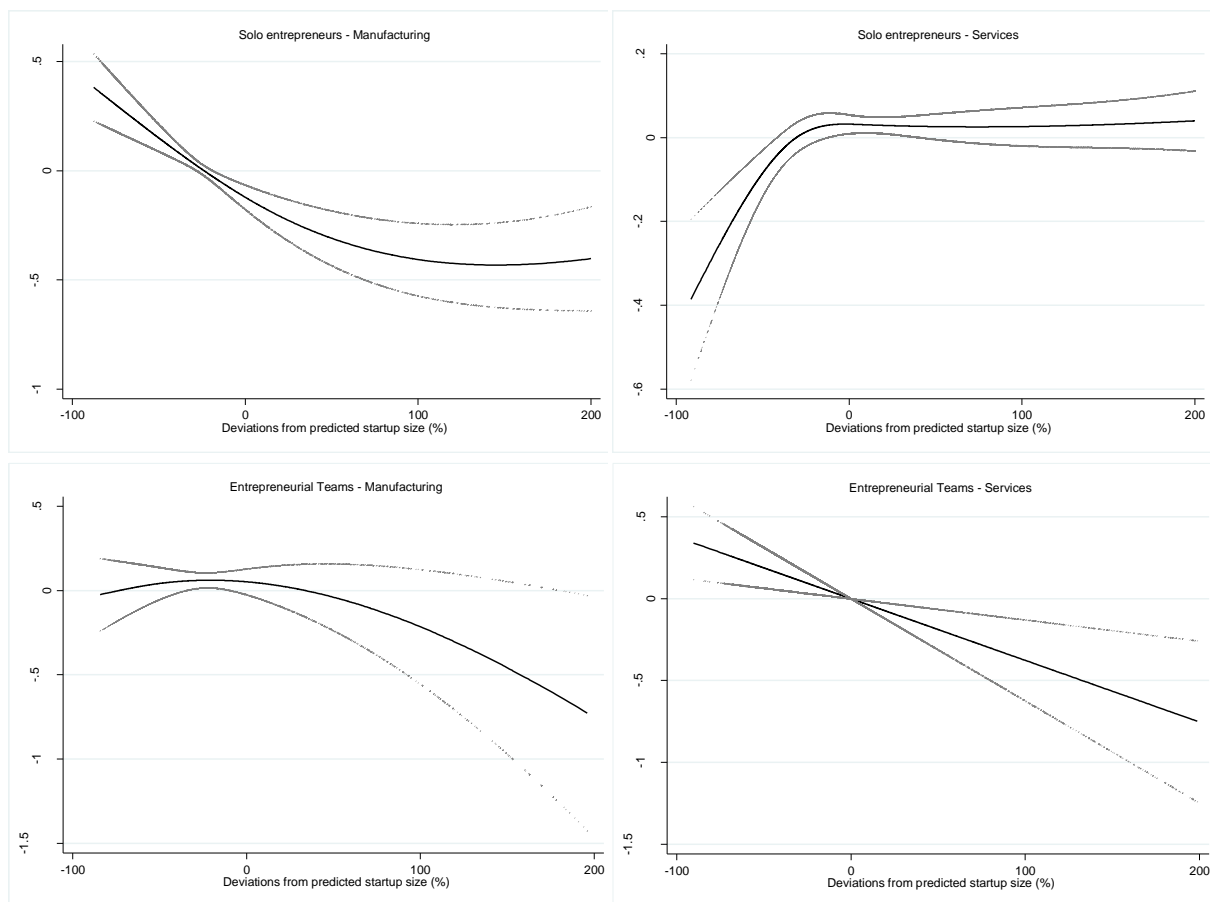
Fig. 3. Estimated relationship between deviations from benchmark startup size and log (relative hazards), by groups of startups (grey lines are 95% pointwise confidence intervals)
