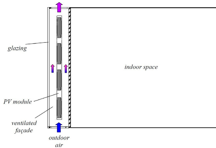
Fig. 2. Schematic of a BIPV system [22]
