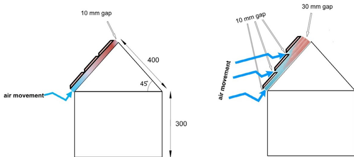
Fig. 8. A stepped layout of BIPV[61].
