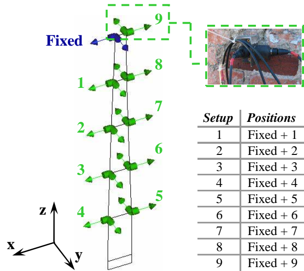
Figure 14: Test setups
