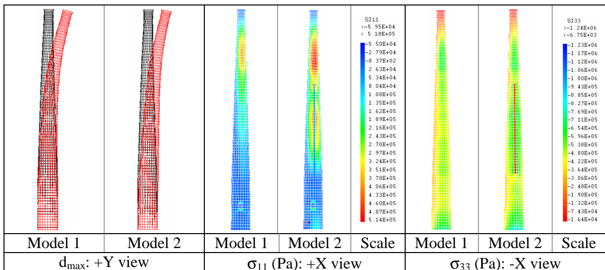
Figure 19: Comparison of seismic analyses results for seismic action type 2
