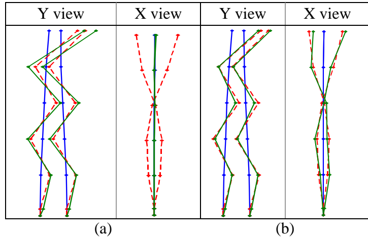
Figure 17: 9 th experimental mode (dashed red) versus numerical mode (green): (a) Model 1; (b) Model 2
