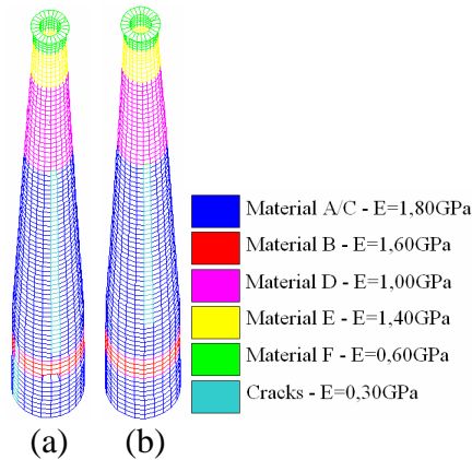
Figure 16: The Young modulus in Model 2: (a) +X view; (b) -X view
