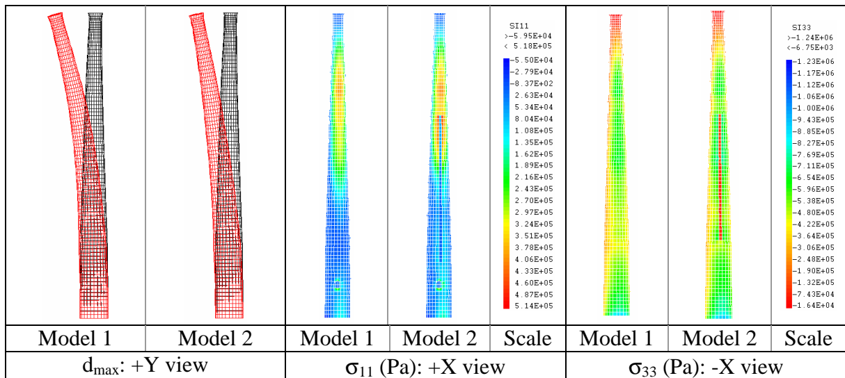
Figure 18: Comparison of the seismic analyses results for seismic action type 1
