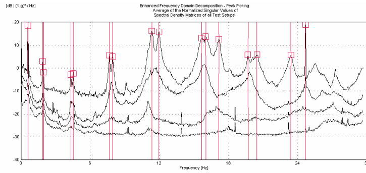
Figure 15: Enhanced frequency domain decomposition peak picking
