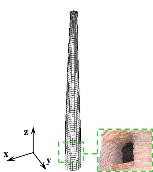
Figure 13: Principal modal directions
