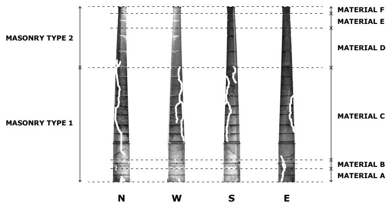
Figure 9: Material and damage identification – North, West, South and East view
