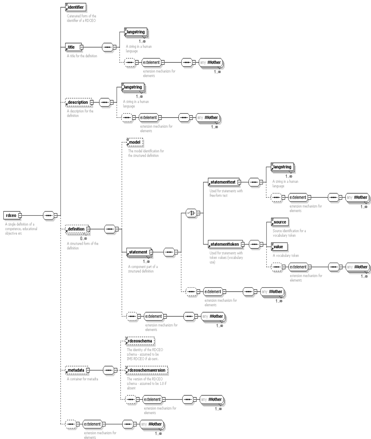
Figure 2. XML schema used as the basis for competency profile template in POOL project (based on http://ltsc.ieee.org/wg20 )
