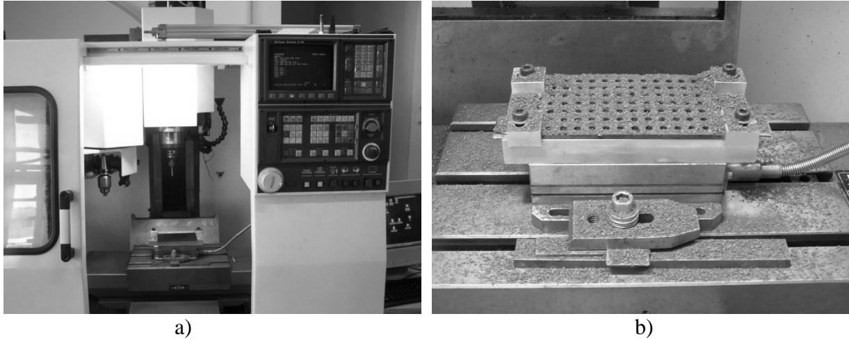
Figure 2 – a) Experimental setup adopted; b) aspect of a drilled plate.
