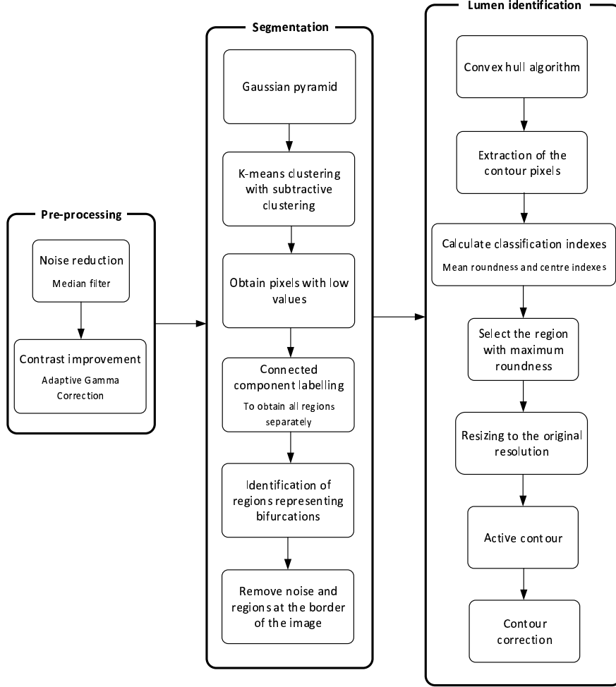
Figure 1: Diagram of the proposed method.
