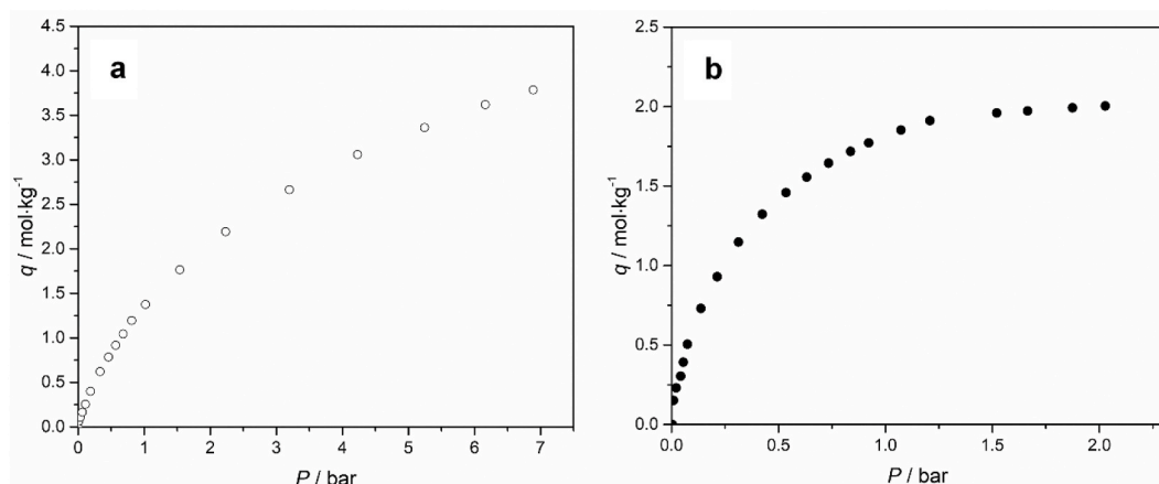
Fig. 5. Adsorption equilibrium isotherms at 25 °C on MFF_8 a) CO 2 and b) SF 6 .
