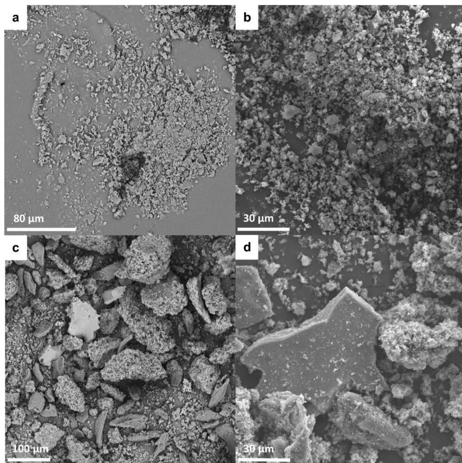
Fig. 2. SEM micrographs with a) 1000 × b) 2000 × of magnification for MFF precursor material and c) 500 × d) 2000 × of magnification for the MFF_8 CMS adsorbent.
