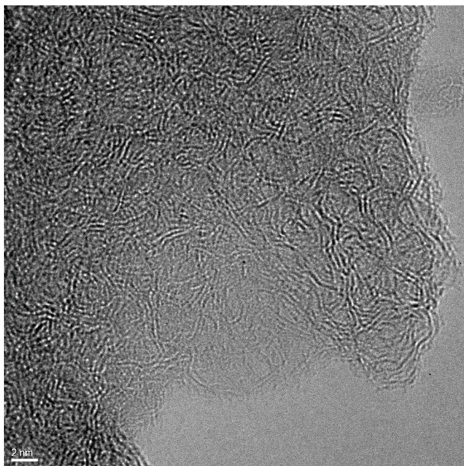
Fig. 8. HRTEM image of a MFF carbon adsorbent carbonized at 1100 °C.
