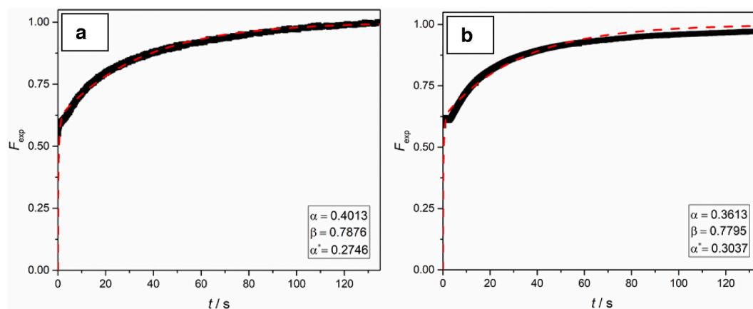
Fig. 10. Experimental uptake curves (black symbols) and fitting model (red dashed lines) for: a) propane and b) propylene. The fitting parameters are also given. (For interpretation of the references to colour in this figure legend, the reader is referred to the Web version of this article.)
