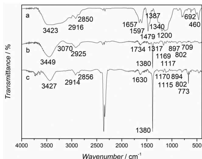
Fig. 4. FTIR spectrum: a) precursor (sample MFF) and; b) sample MFF_2, pre-treated with phosphoric acid and without post-treatment; c) sample MFF_8, pre-treated with phosphoric acid and post-treated with propylene for 12 days.
