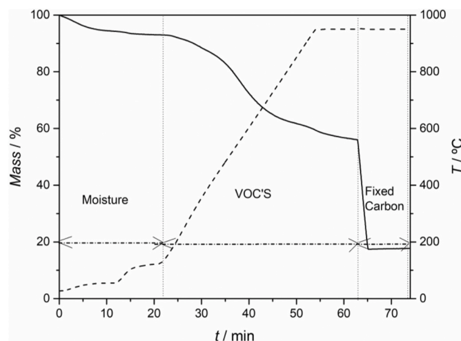
Fig. 1. Proximate analysis of MFF precursor by thermogravimetric method. The removed species at different intervals are identified.
