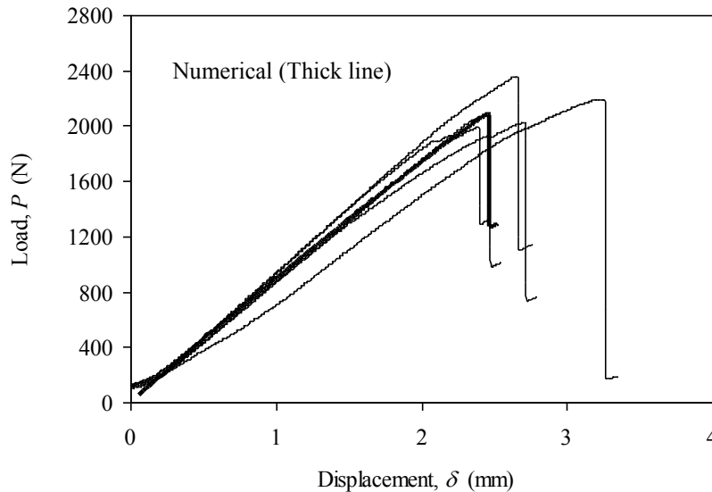
Fig. 8. Numerical and experimental P - \delta curves for repaired beam using thick patch
