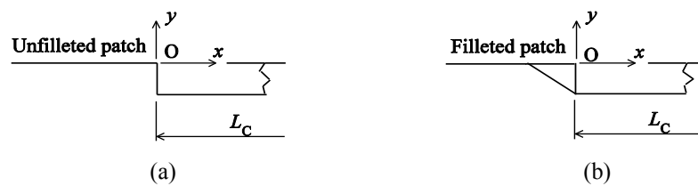
Fig. 4. Geometry of the repaired solutions: (a) unfilleted and (b) filleted patches
