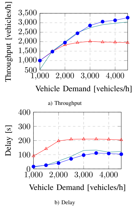
Fig. 10: Intersection management (TL \triangle , FCFS \text{—} , RB \bullet )
