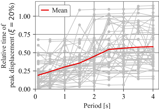
Figure 4. Occurrence of response displacement of elastic systems
