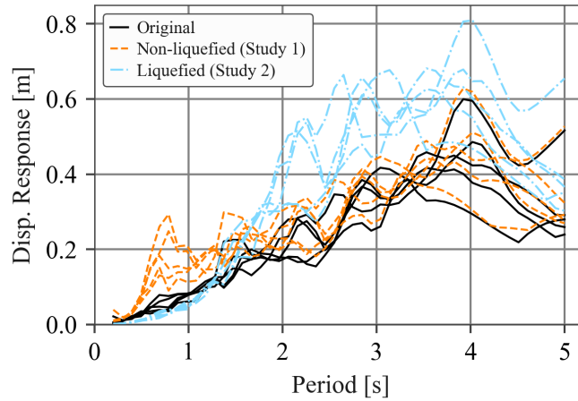
Figure 5. Shift in response spectra due to site effects
