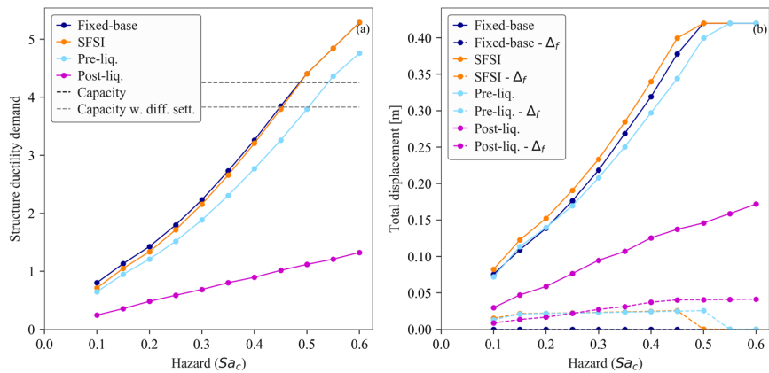
Figure 10. Performance assessment results from case study building
