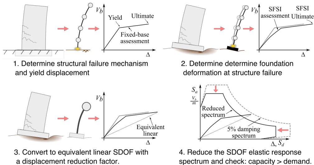
Figure 2. Displacement-based Assessment with SFSI
