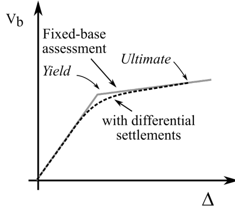
Figure 7. Expected influence of differential settlements on the pushover response of a building
