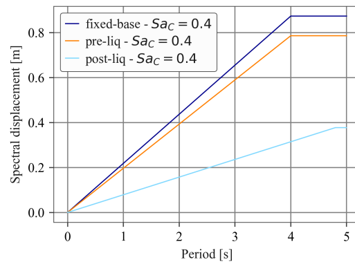
Figure 9. Response spectra for case study building
