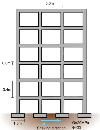
Figure 8. Schematic of the case study building
