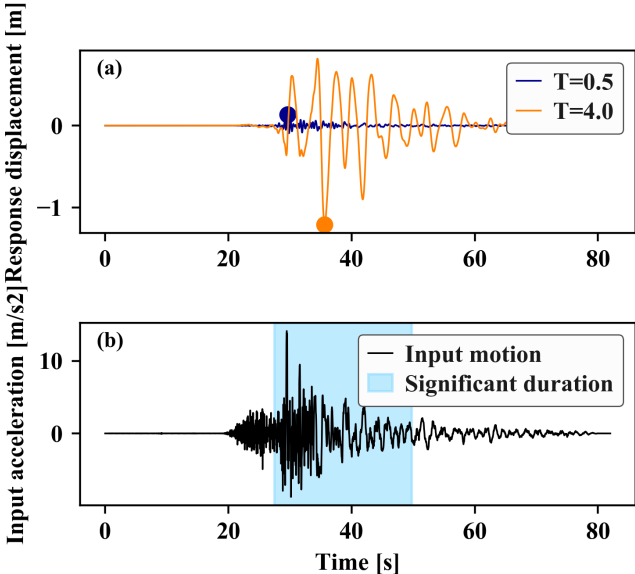
Figure 3. RSN3317_2 motion (a) Response of Elastic systems (b) Time series and significant duration
