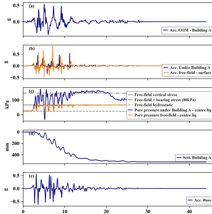
Figure 1. Soil, foundation and structure response from centrifuge experiment SHD02-04 from Dashti et al. (2010)
